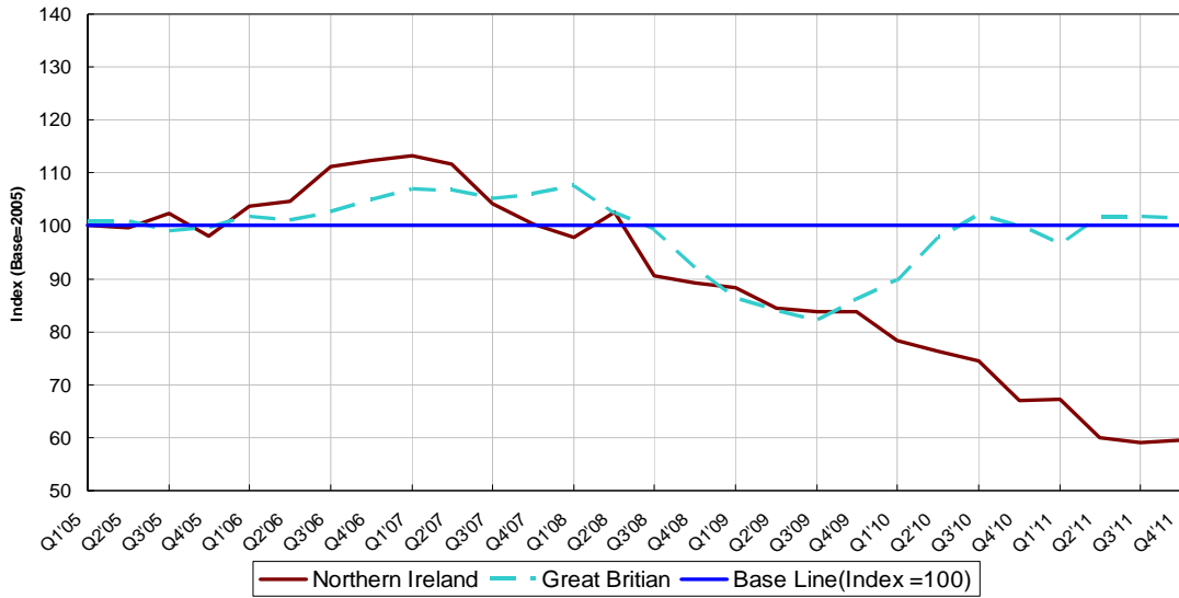
Figure 1.8 Volume of New Work Output NI & GB (Constant (2005) Prices Seasonally Adjusted) Quarters ending March 2005 to December 2011
